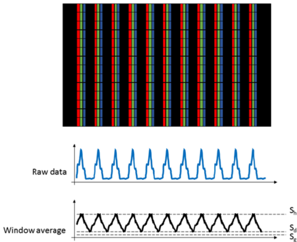
Figure Luminance contrast - characters 1 : Measurement principle (from IDMS 7.2). In summary:
